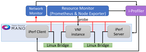
FIGURE 15. VNF setup.
