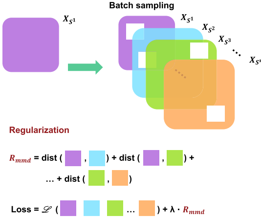
FIGURE 4. An example of data augmentation. X_{S^1} domain (lavender) is the last item in the GAD list for client 1, other domains have more generalization ability. Here, the \text{dist}() method is set as MMD distance.
