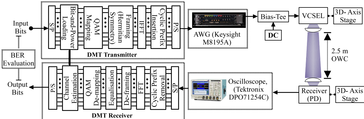
Fig. 1: Schematic diagram of the setup for the VCSEL-based OWC system with DMT modulation and bit-and-power loading
