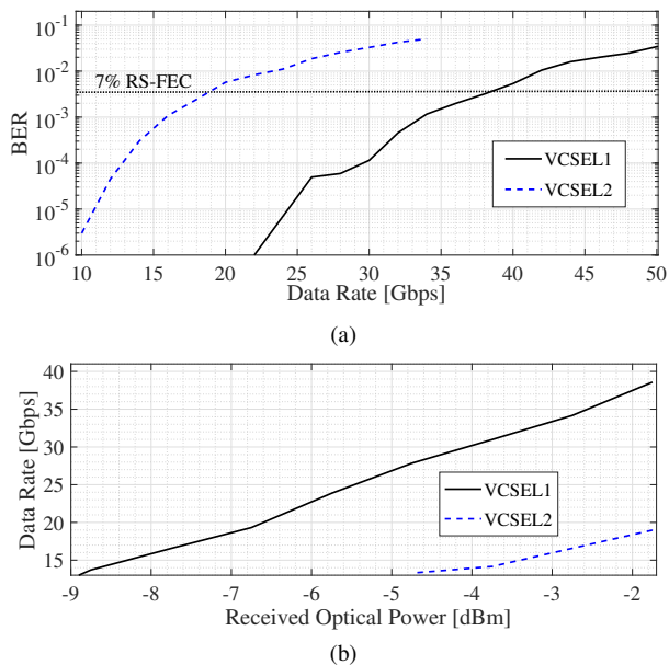
Fig. 4: Plots of: (a) BER versus data rates and (b) Achievable data rates at 7% RS-FEC limit versus received optical power
