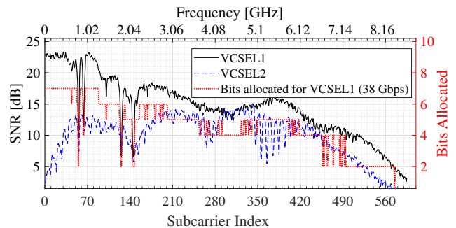
Fig. 3: SNR per sub-carrier from channel estimation. The low-frequency sub-carriers of VCSEL2 have poor SNR performance due to high RIN
