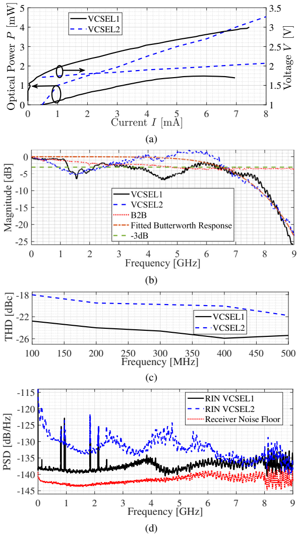
Fig. 2: Measured VCSEL Characteristics: (a) L - I - V Curve (b) Normalised frequency response (c) Total harmonic distortion (THD) and (d) Noise PSD. VCSEL1 denotes the 850 nm SM-VCSEL designed by ICS & CSC; VCSEL2 denotes the commercial 850 nm VCSEL (OPV310).
