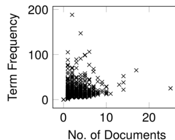
Fig. 1. Keyword statistics
