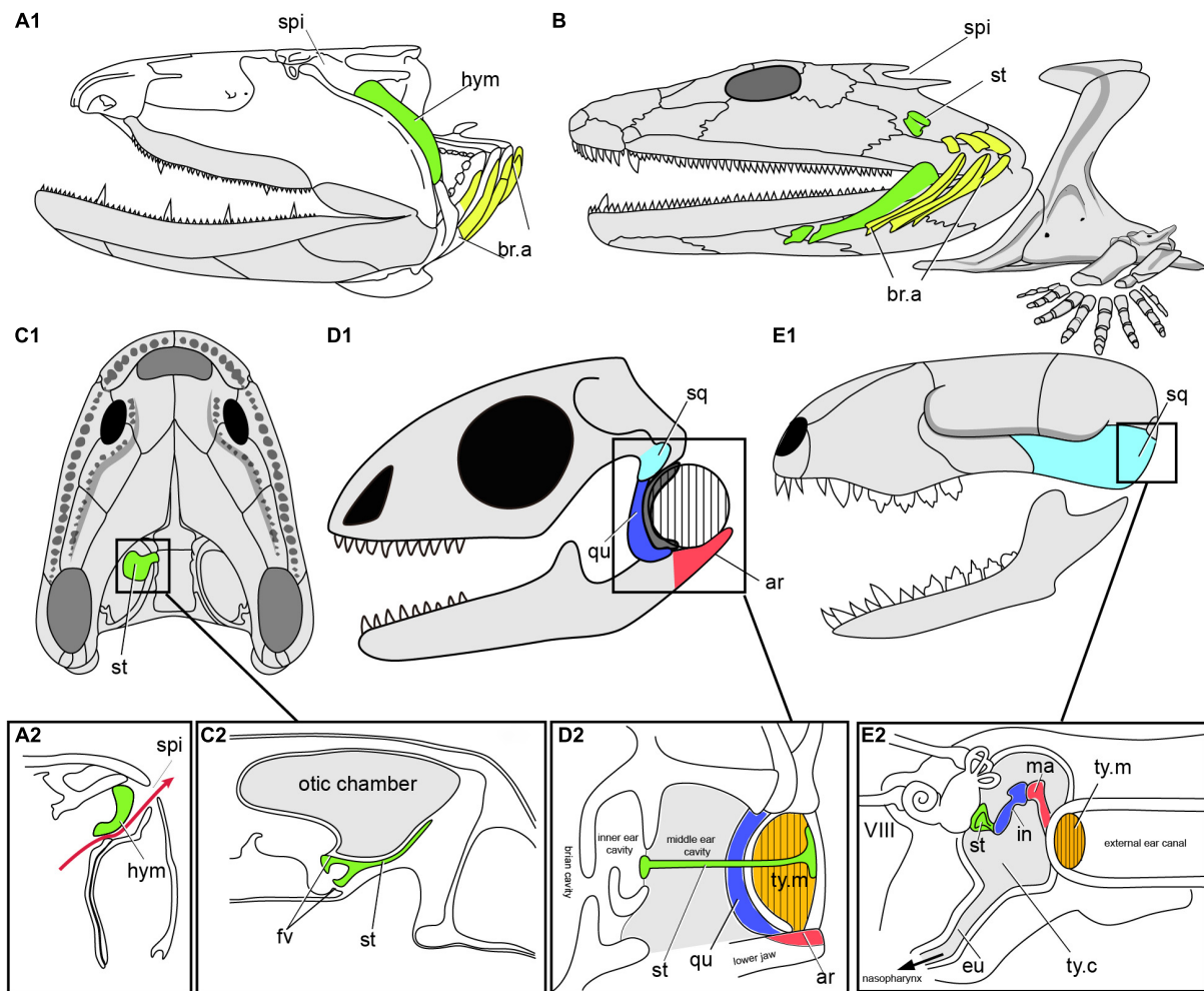
FIGURE 8 | The transition from spiracular pouch of fishes to the middle ear cavity of tetrapods. (A) Fossil osteolepiform Eusthenopteron (A1) , Late Devonian, showing the hyomandibular in the spiracular pouch (A2) , in lateral view, redrawn after (Janvier, 1996b; Brazeau and Ahlberg, 2006). (B) Early tetrapod Acanthostega , Late Devonian of Greenland, showing stapes and the presumed position of the gill arches, in lateral view, redrawn after (Clack et al., 2003; Clack, 2012). (C) Early tetrapod Ichthyostega (C1) , Late Devonian of Greenland, and the reconstructed section (C2) through the air chamber showing its relation to the otic capsule and stapes. (D) Skull of Lizard (D1) , showing the section of middle ear cavity, and the tympanic ear (D2) in reptiles, redrawn after (Clack, 2012). (E) Skull of mammals (E1) , showing the section of middle ear cavity, and the tympanic ear (E2) , redraw after (Farooq et al., 2020). ar, articular; eu, eustachian tube; fv, fenestra vestibuli; hym, hyomandibular; in, incus; ma, malleus; qu, quadrate; sq, squamosal; st, stapes (columella); ty.c, tympanic cavity; ty.m, tympanic membrane (ear drum); other abbreviations as in Figures 1, 2 .
