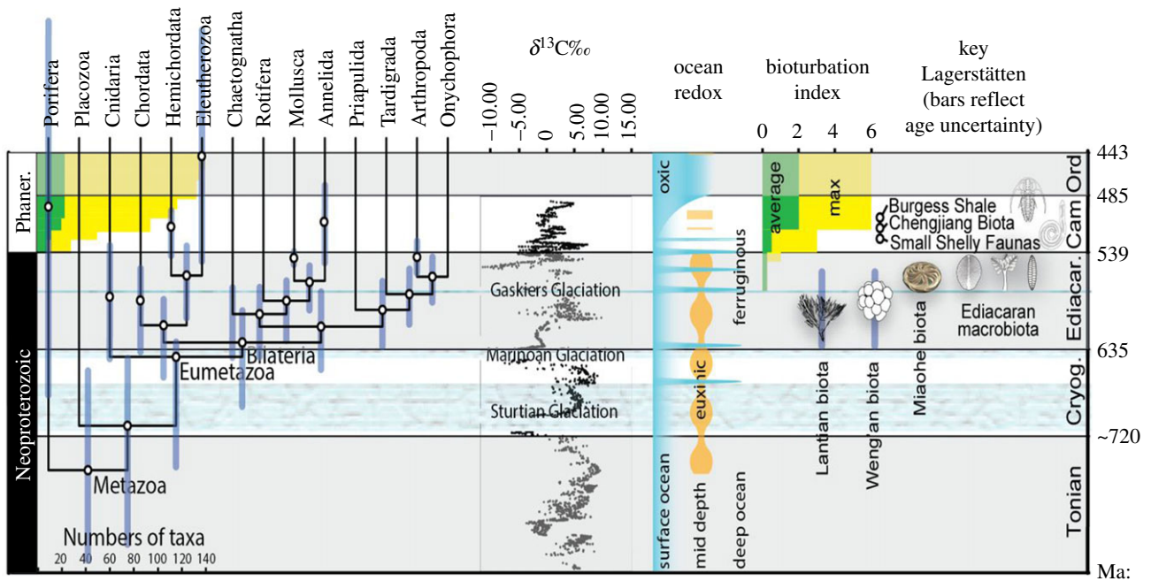
Figure 1. Uncertainty in the timing of the evolution of animals and their environments across the Proterozoic–Phanerozoic transition. From left to right: appearance of animal phyla (green) and classes (yellow) in the fossil record; age uncertainty in the molecular timescale of animal evolution (purple lines); \delta^{13}\text{C} and redox variation—local or global signals?; bioturbation extent, which varies temporally and spatially; Neoproterozoic Lagerstätten, the precise ages of which are extremely uncertain, yielding in turn uncertainty that is reflected in molecular clock estimates of clade age. Data from [4–9].
