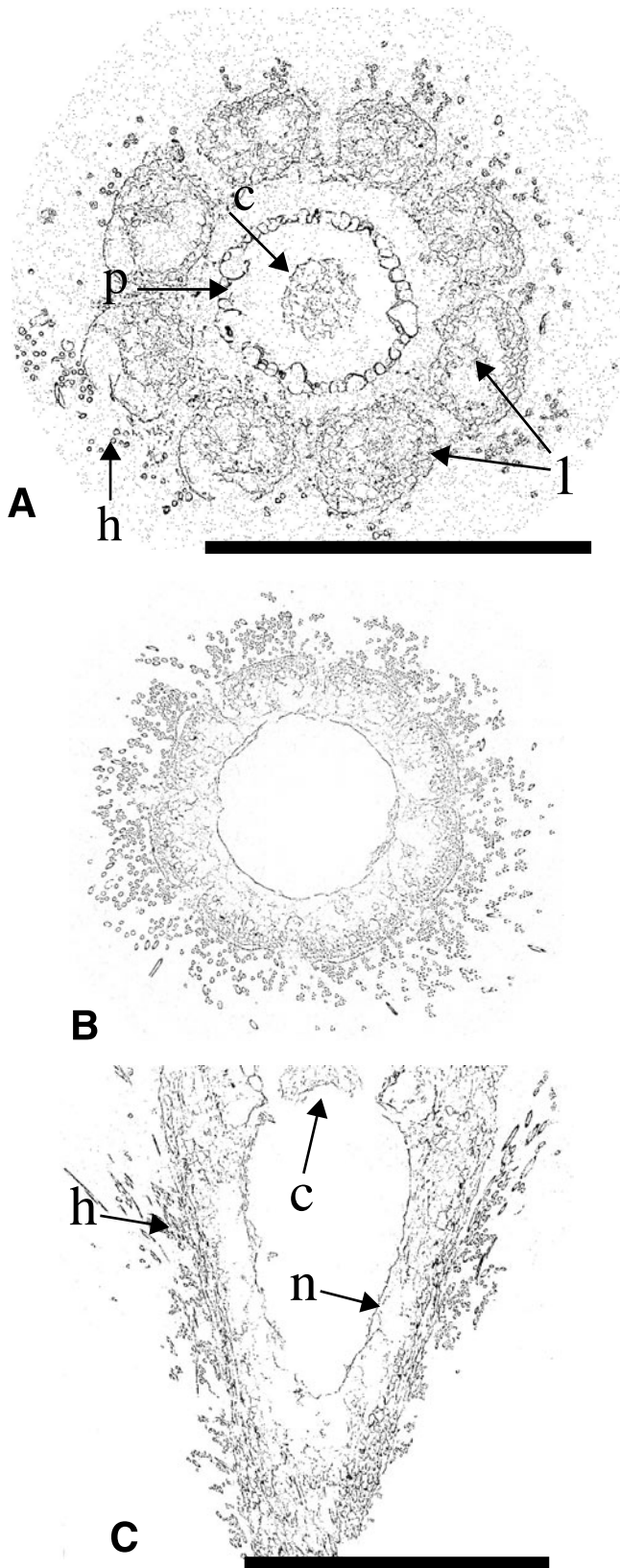
Figure 5. SRXTM of charcoalfied pteridosperm ovule (shown in Fig. 4) from the mid-Mississippian (Carboniferous) of Kingswood, Scotland (from block KIN957I spec 2); scale bar = 1 mm. A: Digital transverse section showing free integumentary lobes (l), central column (c), pollen chamber (p), and hollow external glandular hairs (h). B: Digital transverse section below pollen chamber, showing unlobed integument with external hairs, at same scale as A. C: Digital longitudinal section showing outer glandular hairs (h), central column (c), and nucellus (n).
