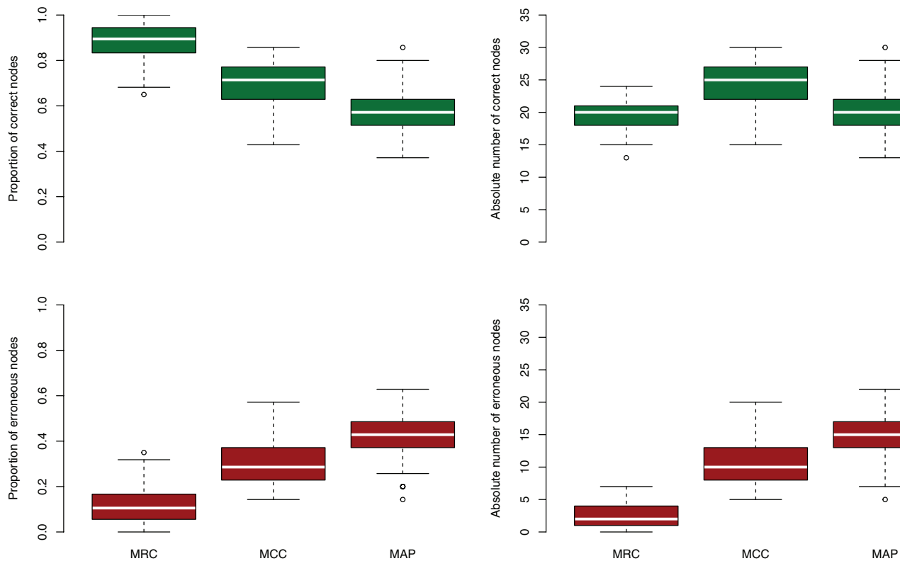
FIGURE 2. The number and proportion of correct and incorrect clades presented in consensus trees constructed from 100 replicate matrices of 100 simulated characters. MCC trees often present more correct nodes than MRC or MAP trees in absolute terms, but they also present many more incorrect nodes than MRC trees in absolute terms. MRC trees present proportionally more correct nodes and fewer incorrect nodes than either MAP or MCC trees.
