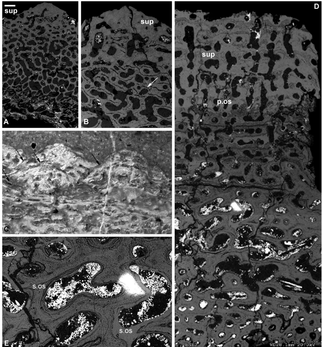
Fig. 3. Histology of the dermal skeleton in the fossil arthrodiran placoderms Antineosteus (A, B) Taemosteus sp. (C) and Dunleosteus terrelli (D, E). SEM images of BRSUG 29371.1 and BRSUG 29371.2 and LM images of NHMUK PV P.33620. Two principal divisions (A) and detail of the superficial and basal layer with cracks running midway between canals probably reflecting cementing lines (B). Appositional growth of superficial layer with truncated and overgrown tubercles (C), principal divisions of a superficial cancellar lamellar layer and a basal cancellar layer (D) and remodelling of the basal cancellous tissue (E). bas, basal lamellar layer; p.os, primary osteon; s.os, secondary osteon; sup, superficial layer. Scale bar equals 300 \mu m in (A), 150 \mu m in (B), 30 \mu m in (C), 200 \mu m in (D), and 100 \mu m in (E).
