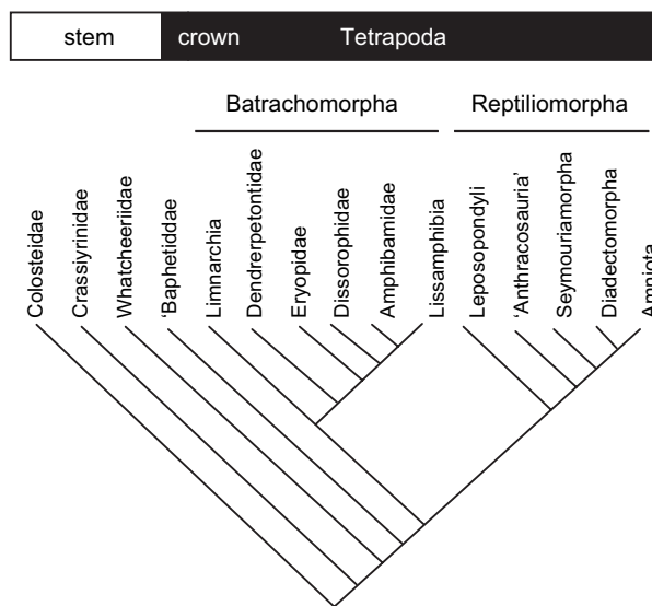
FIG. 6.—Outline relationships of the major clades of Tetrapoda.
