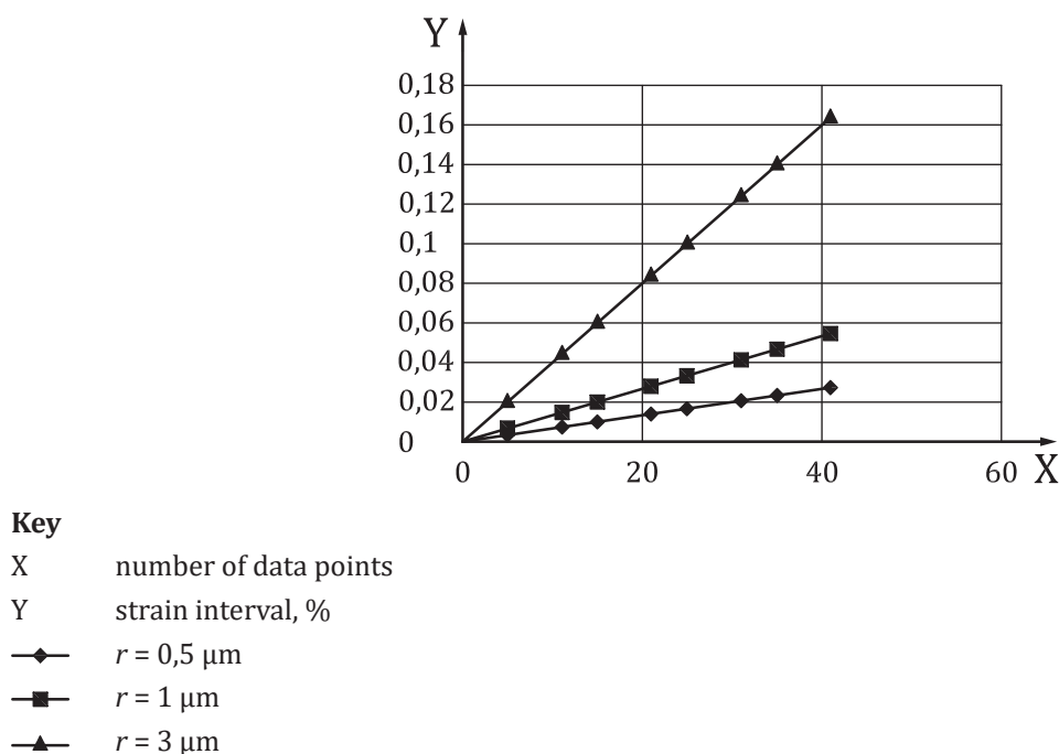
Figure A.1 — Strain interval according to Formula (A.2)
